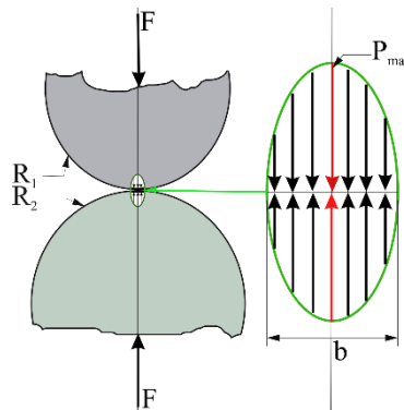
Fig. 3. Contact between two sectioned cylinders, general case
