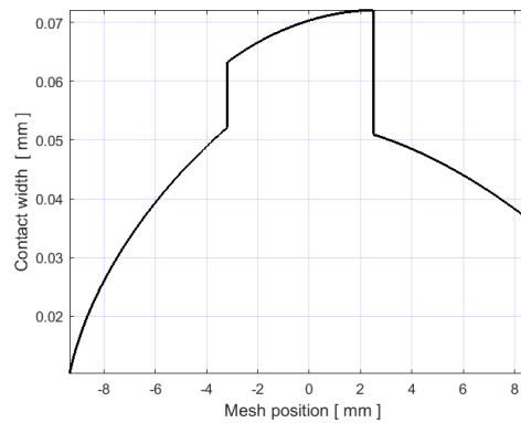
Fig. 4. Contact width.
